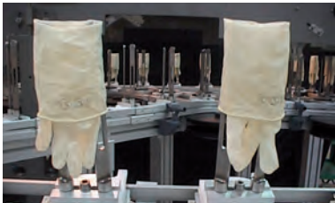
Cuffing mandrels
